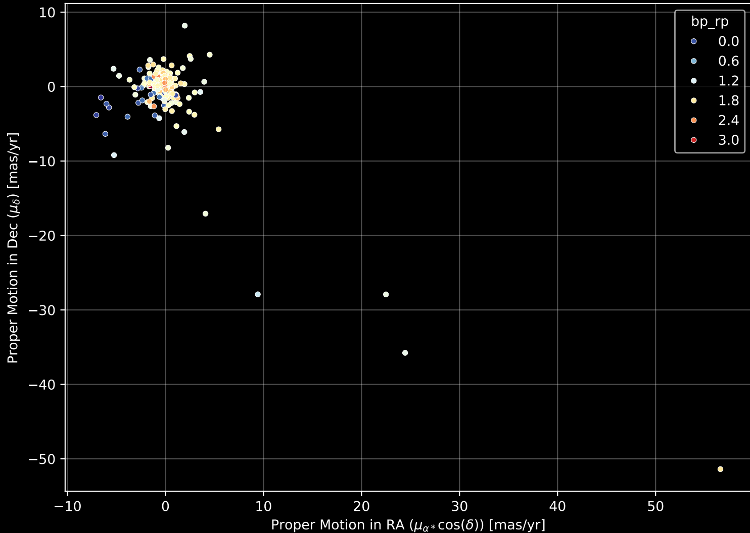
APOGEE DR17 Field: [218-04] Proper Motion Diagram (n= 176)
