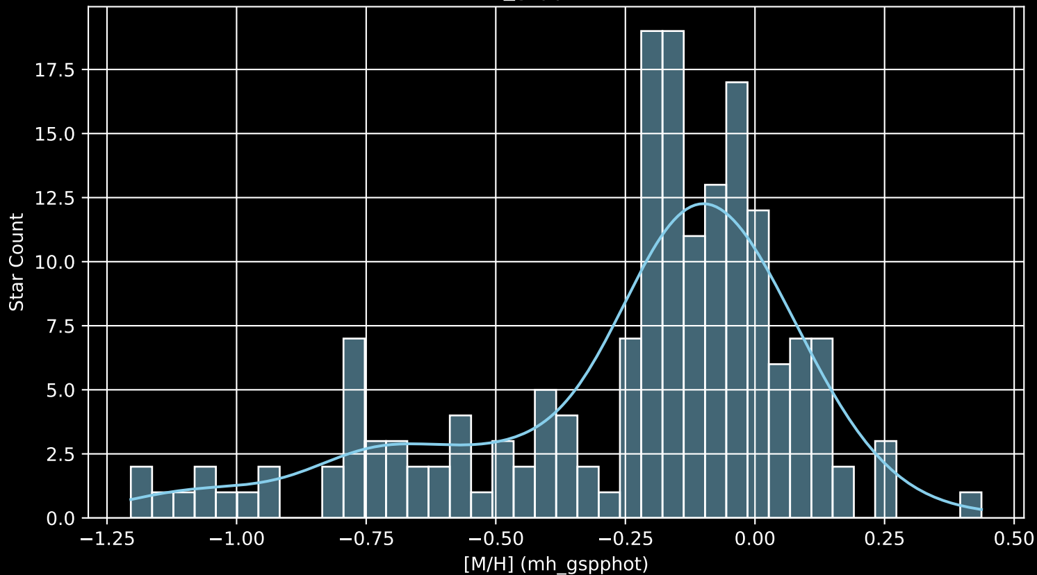
APOGEE DR17 Field: [218-04 [M/H] (mh_gspphot) (n= 175)
