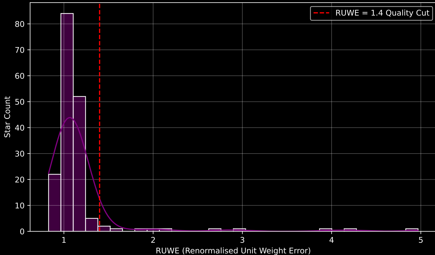
GAPOGEE DR17 Field [218-04] RUWE Distribution (n= 174)
