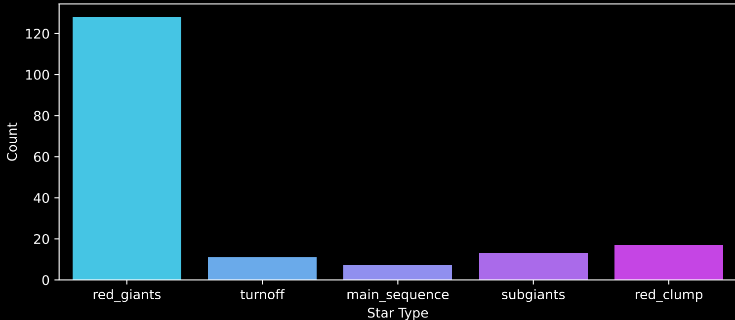
APOGEE DR17 Field: [218-04] Count plot of Star Type
