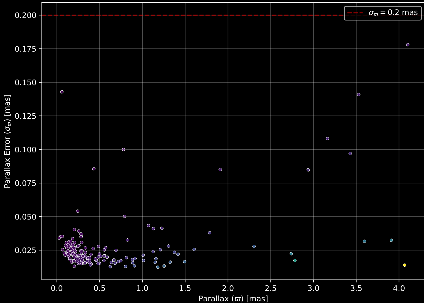
APOGEE DR17 Field: [218-04] Parallax Quality (n= 176)
